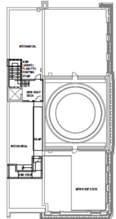
PROPOSED 19th Floor 3:30" = 1" = 0"
